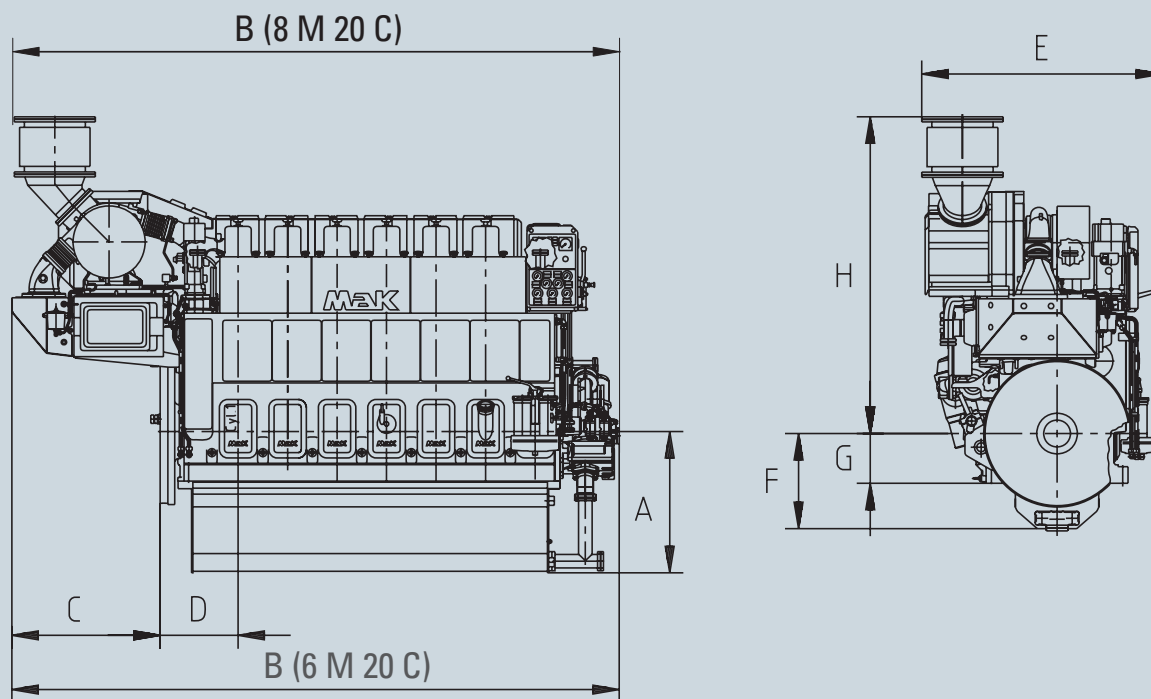
Dimensions (mm) and Weights (t)
